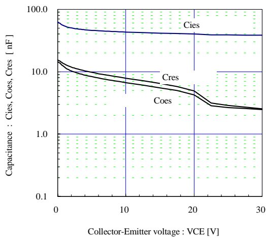
Capacitance vs. Collector-Emmitter voltage (typ.)
