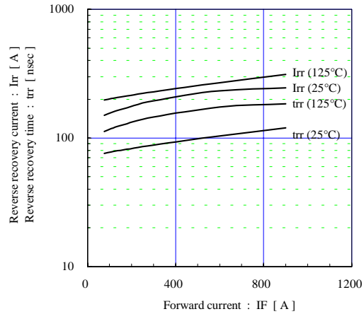
Reverse recovery characteristics (typ.) Vcc=300V, VGE=±15V, Rg=4.7Ω
