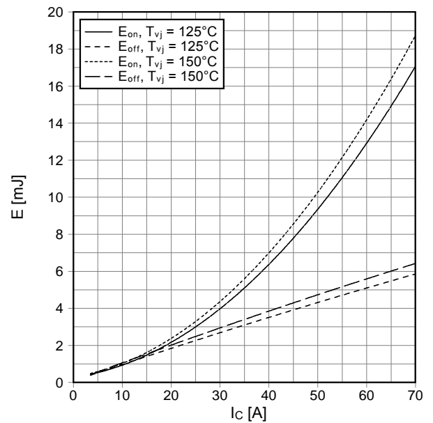
Schaltverluste IGBT-Wechselr. (typisch) switching losses IGBT-inverter (typical) E_{on} = f(I_c) , E_{off} = f(I_c) V_{GE} = \pm 15\text{ V} , R_{Gon} = 27\ \Omega , R_{Goff} = 27\ \Omega , V_{CE} = 600\text{ V}
