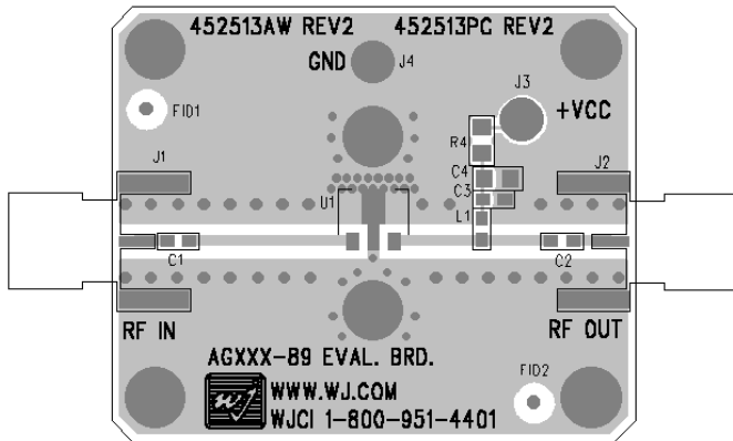
ECG006B-PCB
