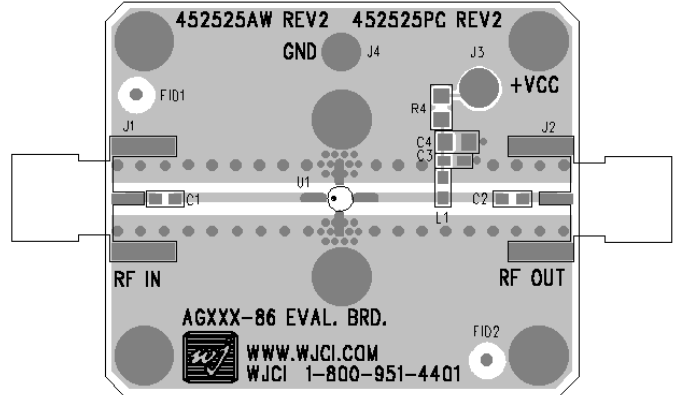
ECG006C-PCB
