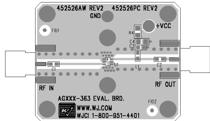
ECG006F-PCB
