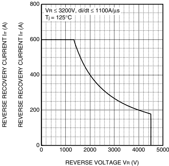
REVERSE RECOVERY SAFE OPERATING AREA (RRSOA)
