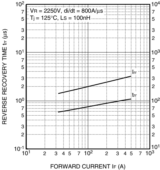
REVERSE RECOVERY CHARACTERISTICS (TYPICAL)
