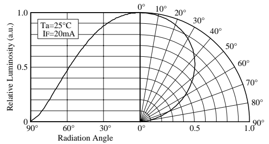
■ Directivity (NSCG455A)
