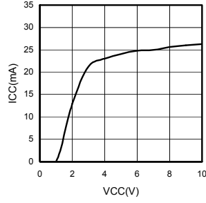
Fig.5 Circuit Current - Supply Voltage (BD3402KS2)
