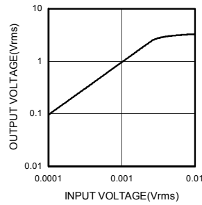
Fig.17 Output Voltage – Input Voltage (PB)
