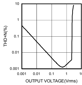
Fig.8 Total Harmonic Distortion ratio - Output Voltage
