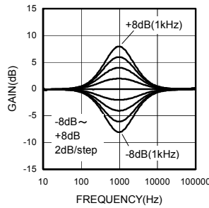
Fig.11 Middle Gain - Frequency (BD3401KS2)
