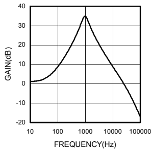
Fig.22 AMS Gain - Frequency (BD3401KS2)
