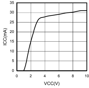
Fig.4 Circuit Current - Supply Voltage (BD3401KS2)
