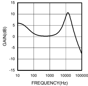
Fig.19 Amp Gain - Frequency (REC)
