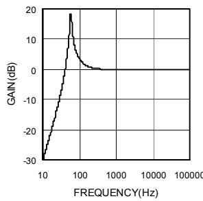
Fig.13 Bass Boost Gain - Frequency (BD3401KS2)
