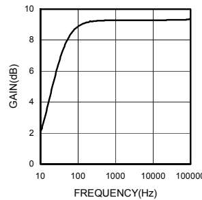
Fig.14 Surround Gain - Frequency (BD3401KS2)
