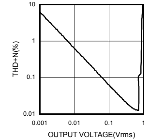
Fig.21 Total Harmonic Distortion ratio – Output Voltage (REC)
