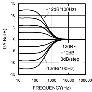
Fig.10 Bass Gain - Frequency (BD3402KS2)
