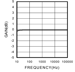
Fig.6 Voltage Gain - Frequency
