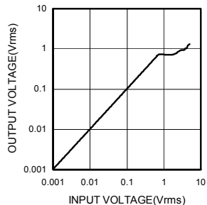
Fig.20 Output Voltage – Input Voltage (REC)
