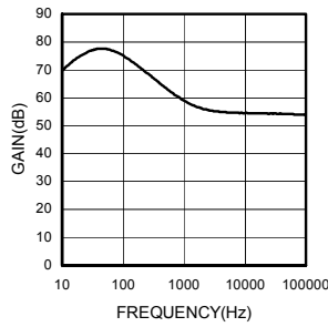
Fig.16 Amp Gain - Frequency (PB)
