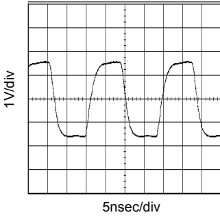
Fig.1 54MHz output waveform (VDD=3.3V,CL=15pF,Ta=25°C)
