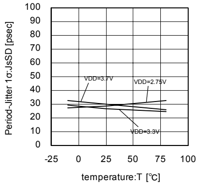
Fig.72 49.5MHz Period-Jitter 1 \sigma temperature characteristics
