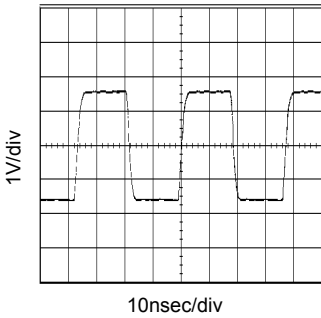
Fig.4 27MHz output waveform (VDD=3.3V,CL=15pF,Ta=25°C)
