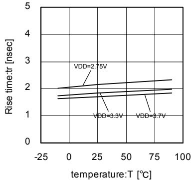
Fig.85 78MHz Rise-time temperature characteristics
