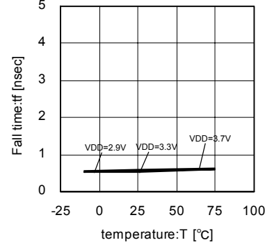
Fall-time temperature characteristics
