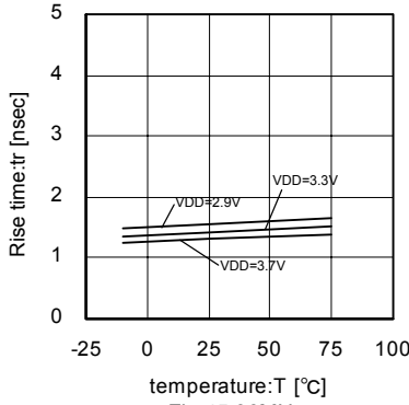
Fig. 45 36MHz Rise-time temperature characteristics
