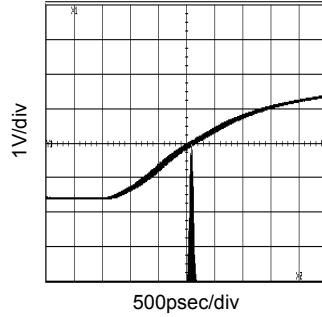
Fig.2 54MHz Period-Jitter (VDD=3.3V,CL=15pF,Ta=25°C)
