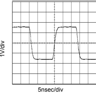
Fig.7 36MHz output waveform (VDD=3.3V,CL=15pF,Ta=25°C)
