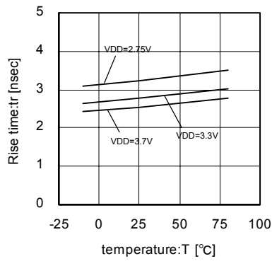
Fig.75 36MHz Rise-time temperature characteristics
