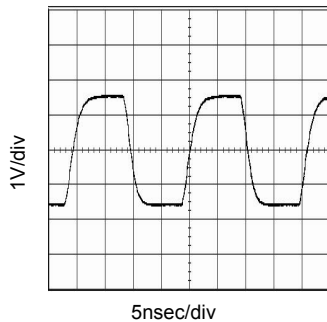
Fig.28 48MHz output waveform (VDD=3.3V,CL=15pF,Ta=25°C)
