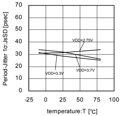
Fig.77 36MHz Period-Jitter 1 \sigma temperature characteristics
