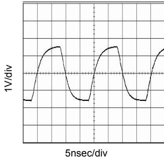
Fig.22 49.5MHz output waveform (VDD=3.3V,CL=15pF,Ta=25°C)
