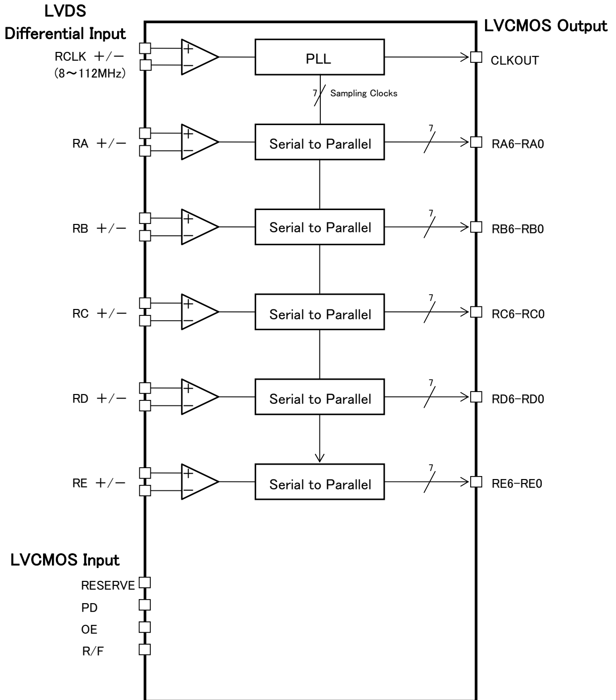
Figure-1 Block Diagram
