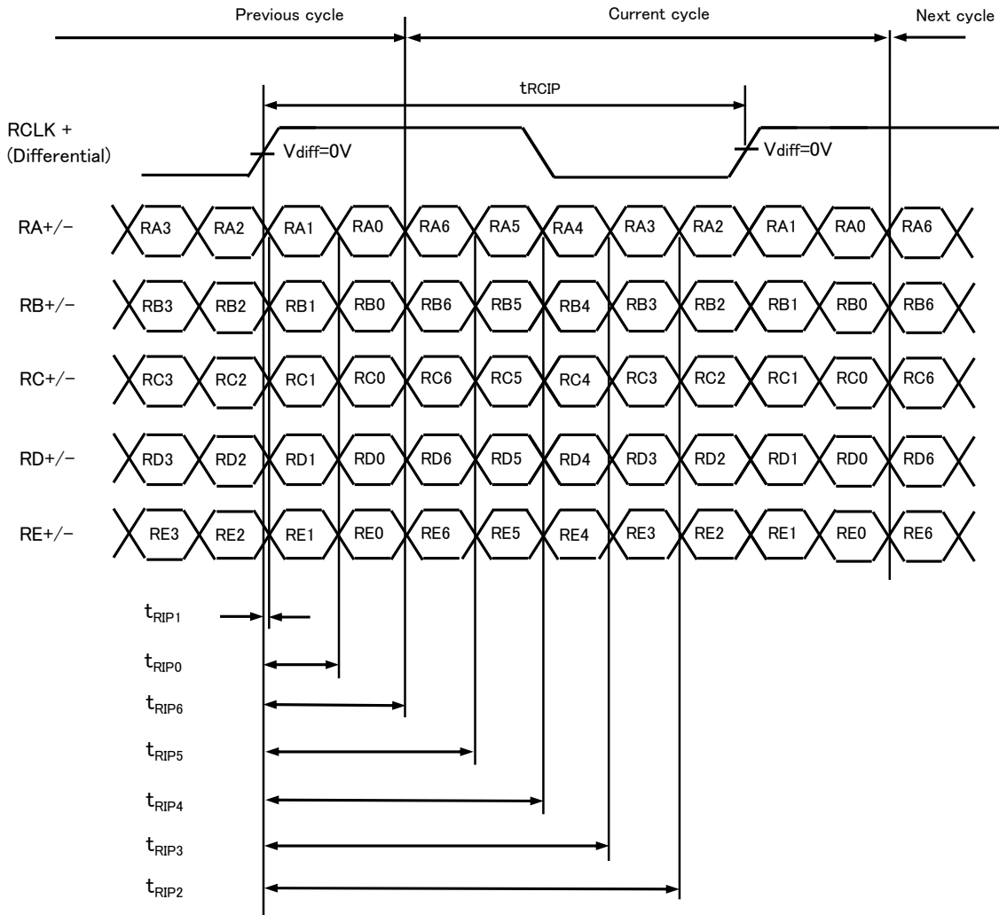
Figure-8 LVDS data and clock input timing
