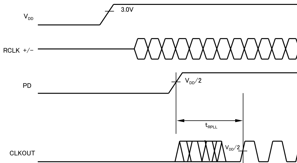
Figure-7 Phase-Locked Loop set time
