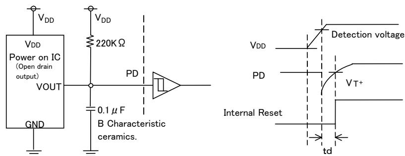
Figure-12 Power on reset by specific IC
