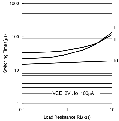
Switching Time vs. Load Resistance (Ta=25°C)
