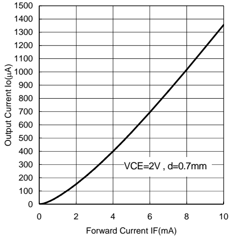
Output Current vs. Forward Current ( T_a=25^\circ\text{C} )
