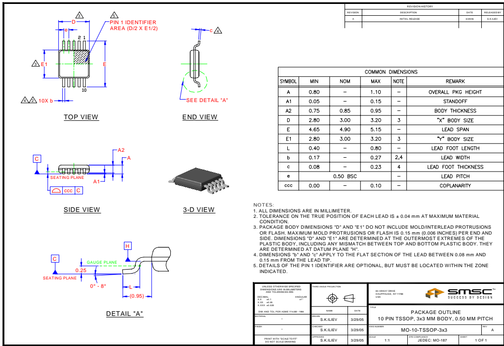
Figure 1 EMC1152 10-Pin MSOP Package Drawing
