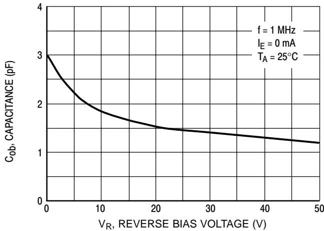
Figure 19. Output Capacitance
