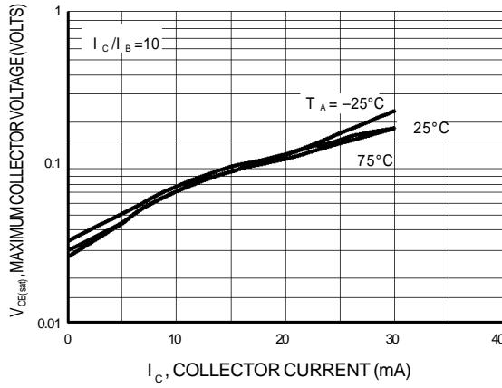
Figure 12. V_{CE(sat)} versus I_C
