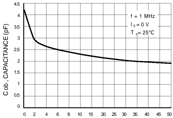
Figure 19. Output Capacitance
