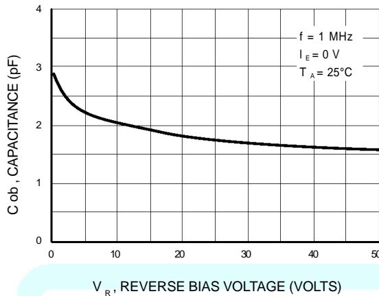
Figure 9. Output Capacitance
