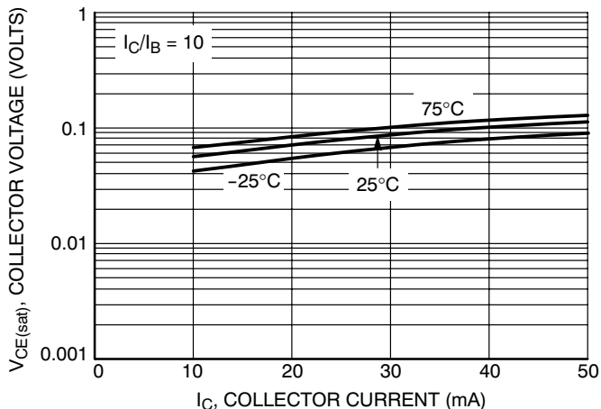
Figure 42. V_{CE(sat)} versus I_C
