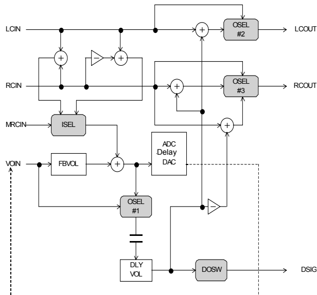
Fig.31 Input mixer selector circuit
