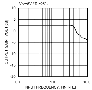
Fig.6 A/D frequency characteristic
