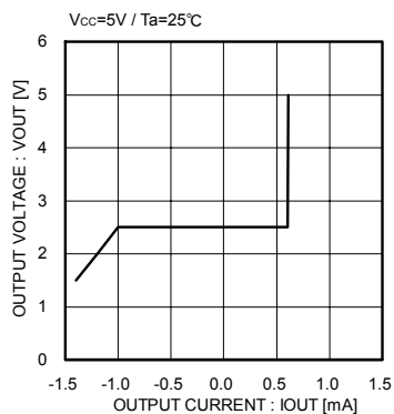
Fig.10 LPF operation amplifier output performance
