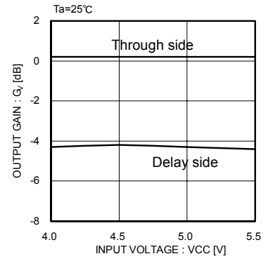
Fig.3 Total gain characteristic
