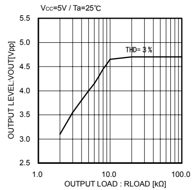
Fig.9 Through side output load drive characteristic
