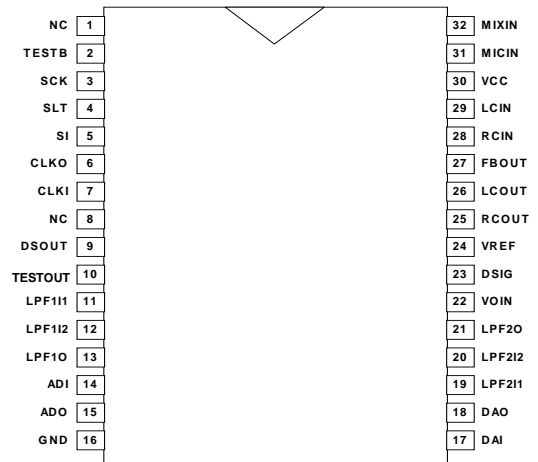
Fig.29 Pin assignment
