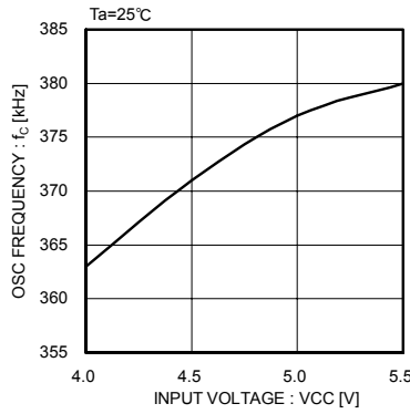
Fig.2 Oscillation frequency
