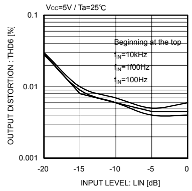
Fig.18 Line amplifier distortion characteristic
