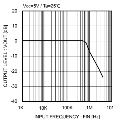
Fig.8 MIX operation amplifier frequency characteristic
