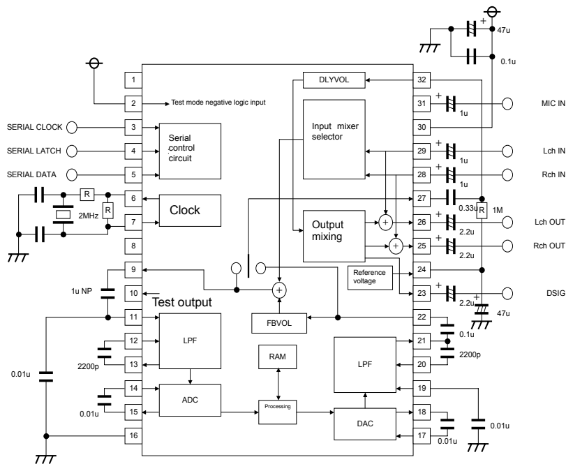
Fig.30 Application circuit
