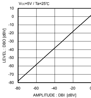
Fig.19 MIX VOL linearity
