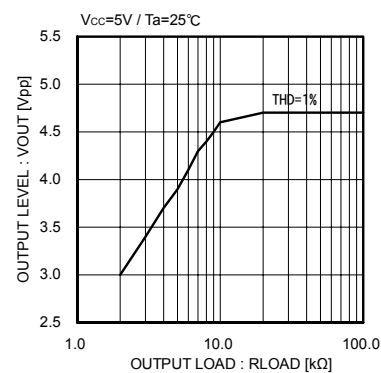
Fig.12 Delay side output load drive characteristic
