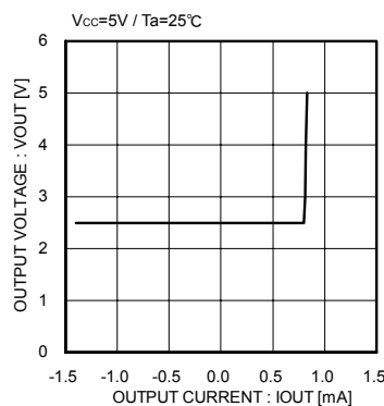
Fig.11 MIX operation amplifier output performance
