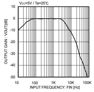
Fig.15 FBVOL frequency characteristic
