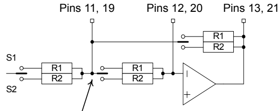
Fig.32 Input LPF / Output LPF circuit
