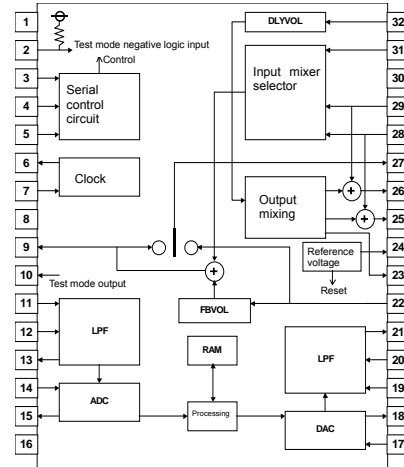
Fig.28 Block diagram
