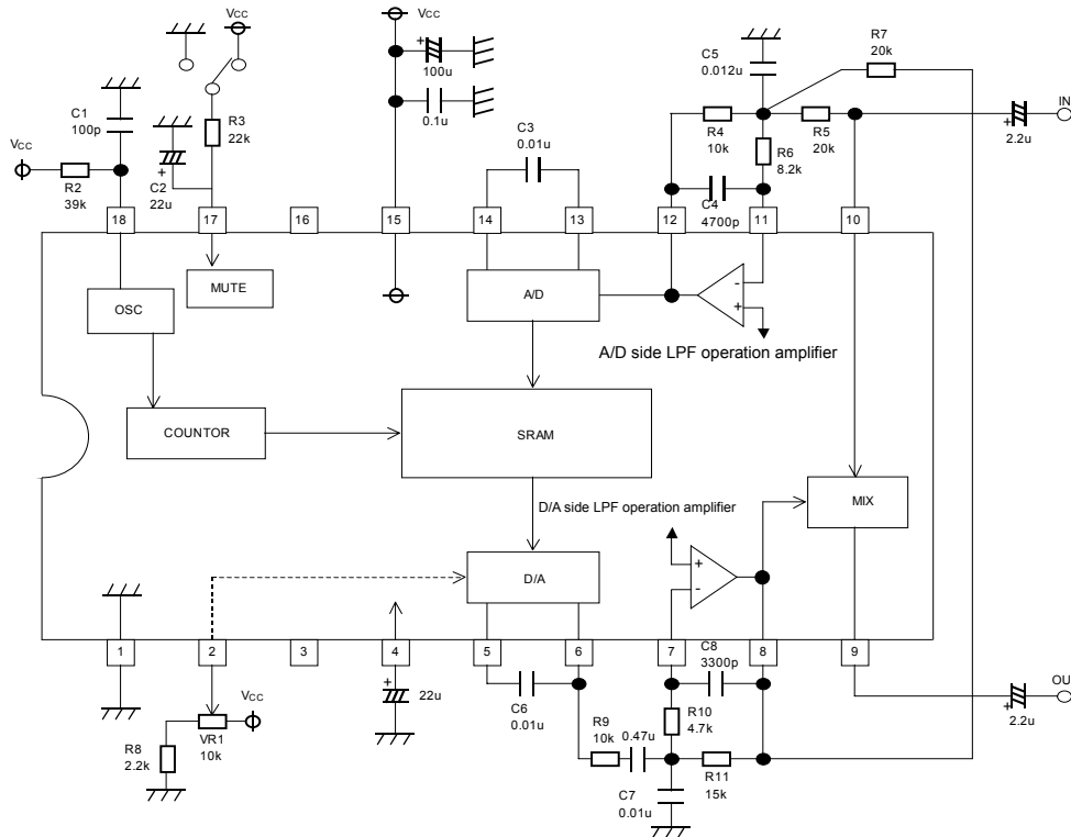
Fig.27 Application circuit
