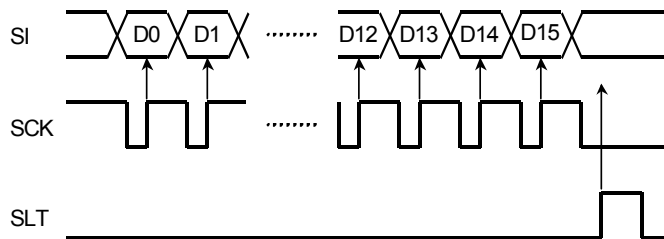
Fig.33 Serial interface specification
