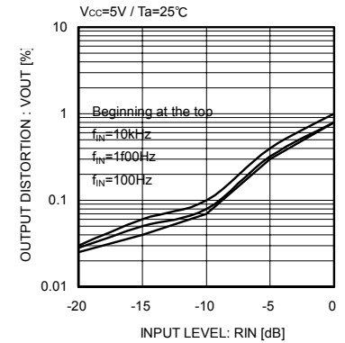
Fig.21 MIX VOL distortion characteristic
