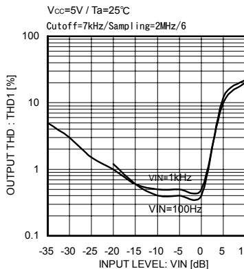
Fig.22 Input level vs distortion ratio characteristic 1
