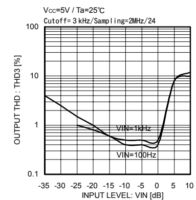
Fig.24 Input level vs distortion ratio characteristic 3
