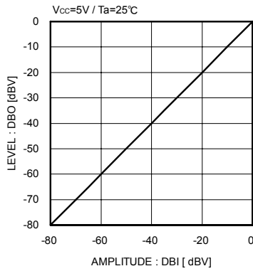
Fig.16 Line amplifier linearity
