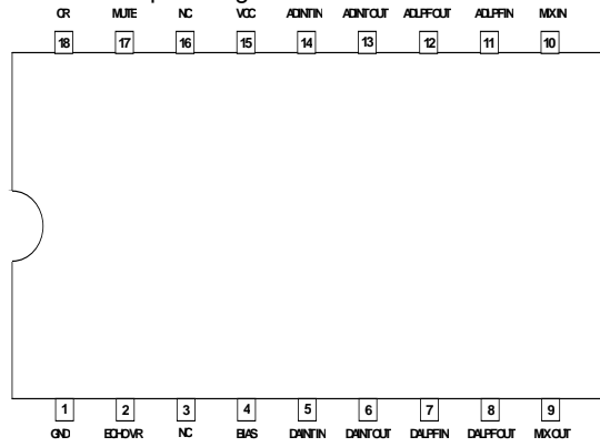
Fig.25 BU9253AS pin assignment
