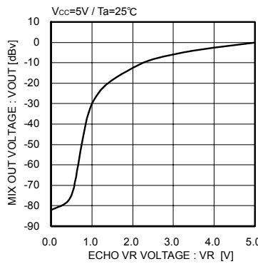
Fig.5 ECHO VR characteristic
