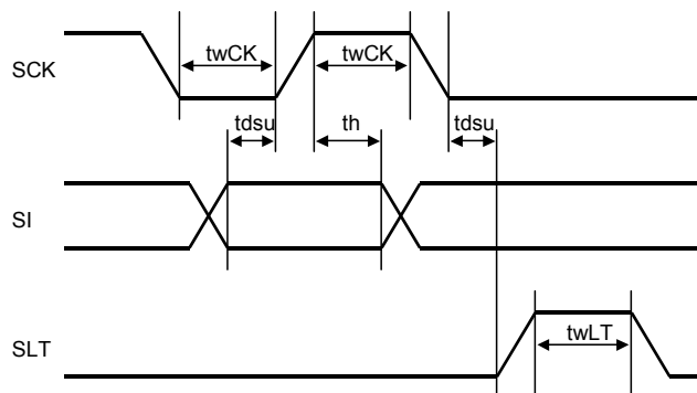
Fig.34 Serial timing
