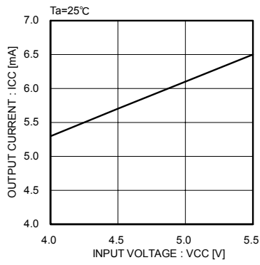
Fig.1 Current consumption
