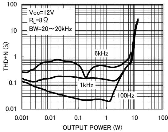
Fig. 1 THD+N - Output power
