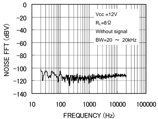
Fig. 12 FFT of Output Noise Voltage
