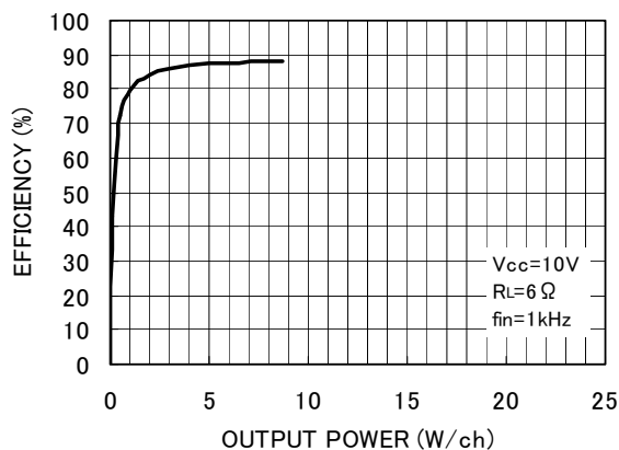
Fig. 19 Efficiency - Output power
