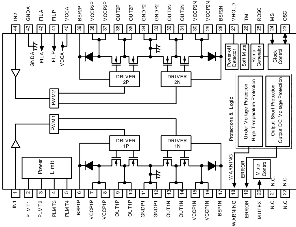
Fig. 28 Pin Assignment Diagram
