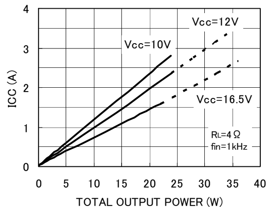
Fig. 27 Current consumption - Output power
