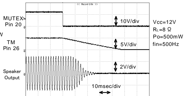
Fig. 14 Wave form when Activating Soft-mute
