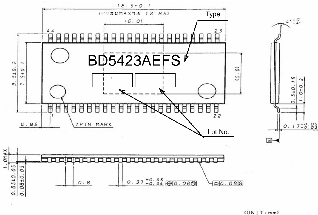
Fig. 29 Outer Dimensions and Inscriptions of HTSSOP-A44 Package
