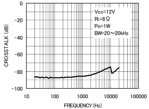
Fig. 4 Crosstalk - Frequency
