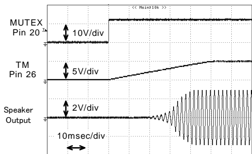
Fig. 13 Wave form when Releasing Soft-mute
