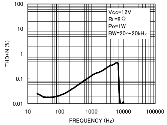
Fig. 2 THD+N - Frequency
