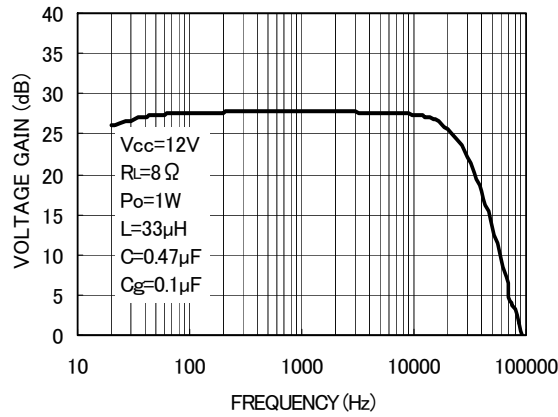
Fig. 3 Voltage gain - Frequency
