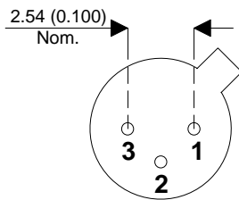
TO-18 (TO-206AA)
