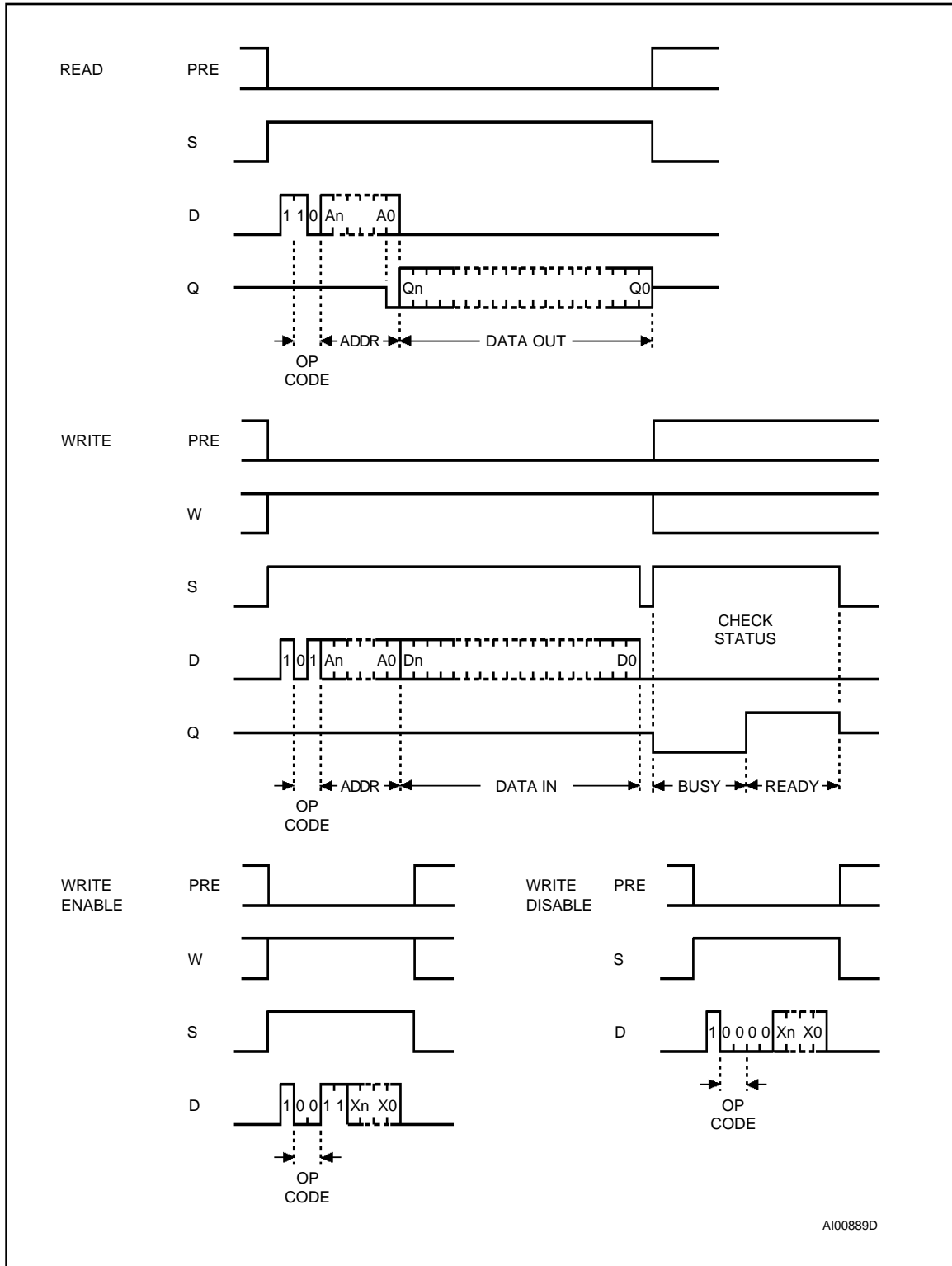
Figure 6. READ, WRITE, WEN, WDS Sequences
