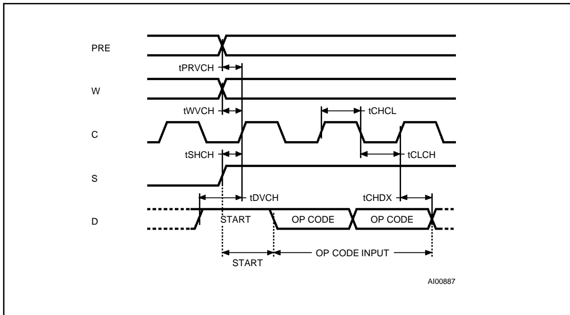
Figure 4. Synchronous Timing, Start and Op-Code Input
