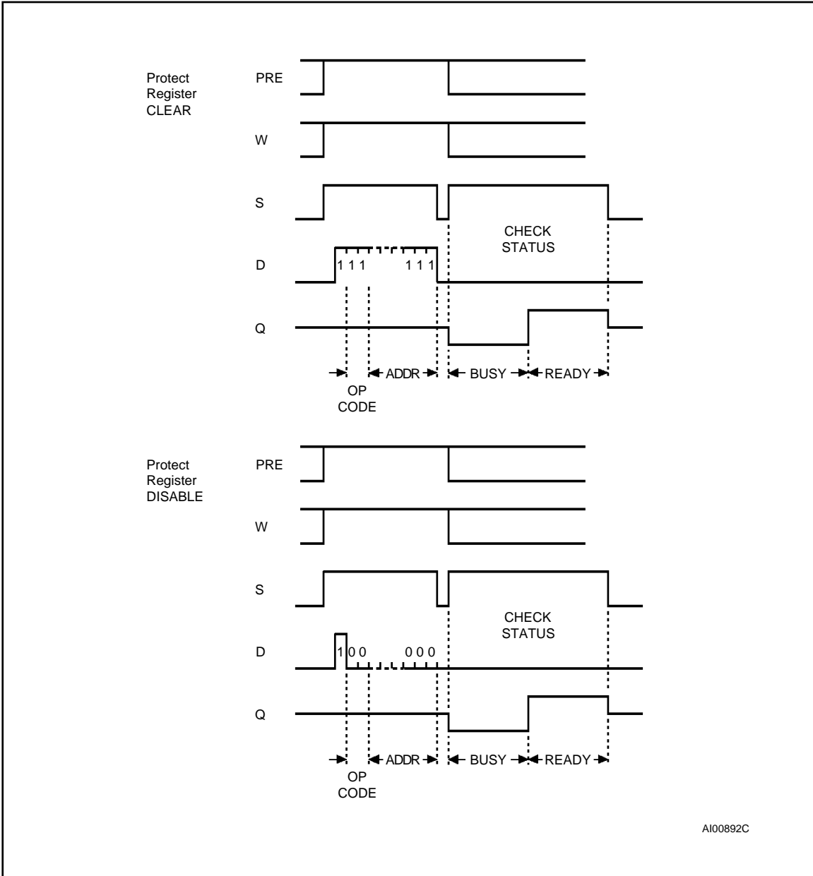
Figure 9. PRCLEAR, PRDS Sequences
