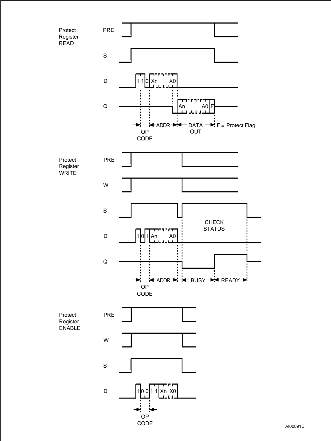
Figure 8. PRREAD, PRWRITE, PREN Sequences
