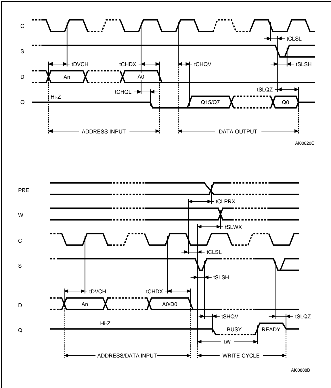
Figure 5. Synchronous Timing, Read or Write
