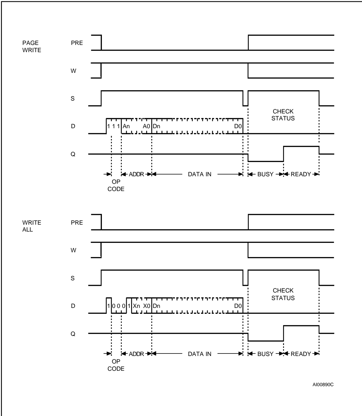
Figure 7. PAWRITE, WRALL Sequences
