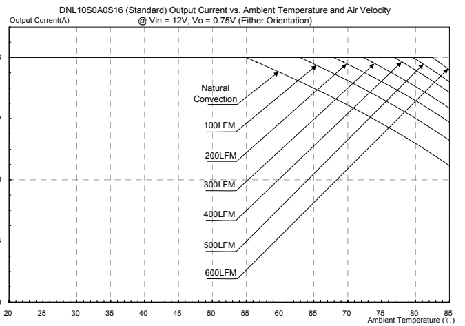
Figure 35: DNL10S0A0S16 (Standard) Output current vs. ambient temperature and air velocity @ Vin=12V, Vo=0.75V(Either Orientation)
