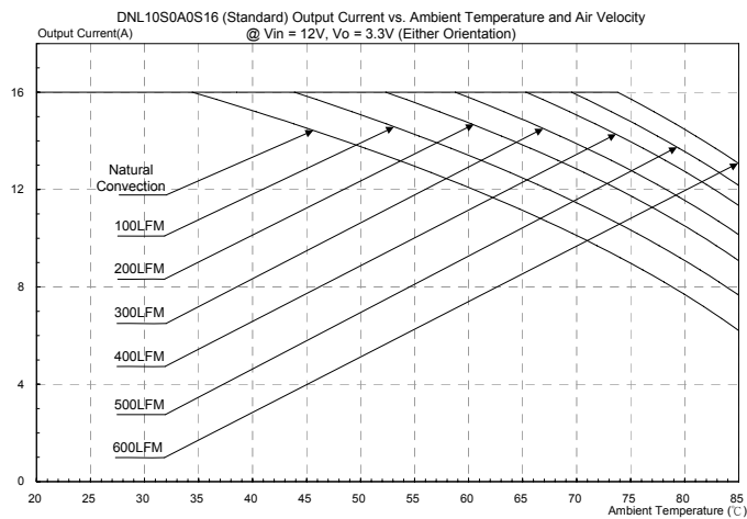
Figure 33: DNL10S0A0S16 (Standard) Output current vs. ambient temperature and air velocity @ Vin=12V, Vo=3.3V(Either Orientation)
