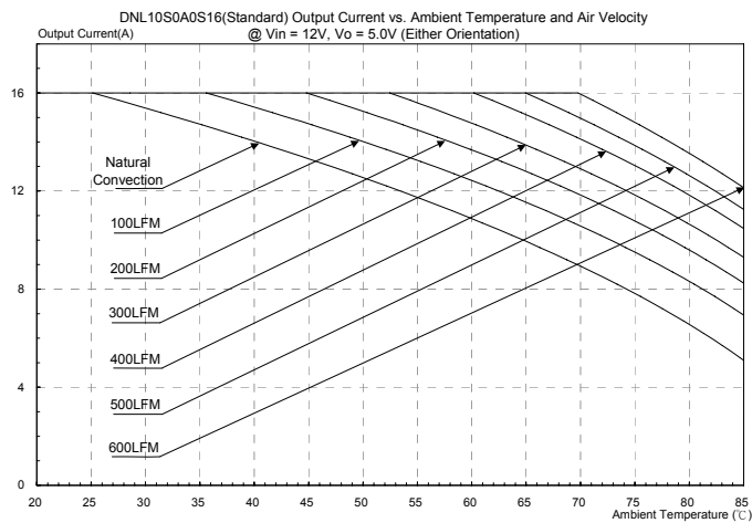
Figure 32: DNL10S0A0S16 (Standard) Output current vs. ambient temperature and air velocity @ Vin=12V, Vo=5.0V(Either Orientation)
