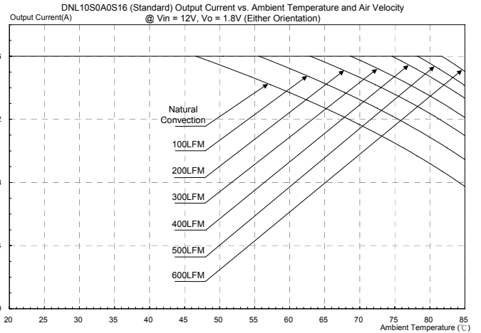
Figure 34: DNL10S0A0S16 (Standard) Output current vs. ambient temperature and air velocity @ Vin=12V, Vo=1.8V(Either Orientation)
