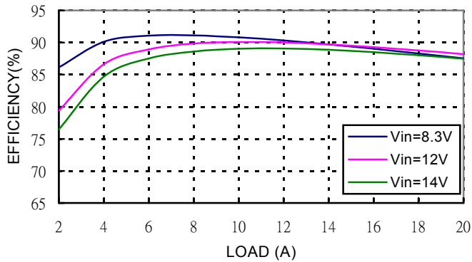
Figure 1: Converter efficiency vs. output current (0.75V output voltage)
