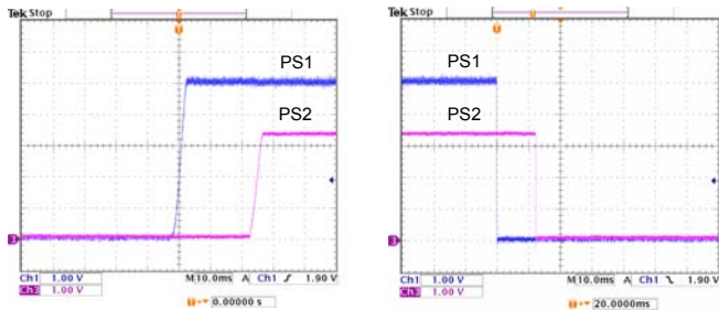
Figure 35: Sequential start-up
