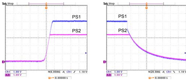
Figure 36: Simultaneous
