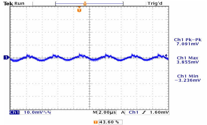
Figure 8: Output ripple & noise at 12Vin, 1.2V/20A out
