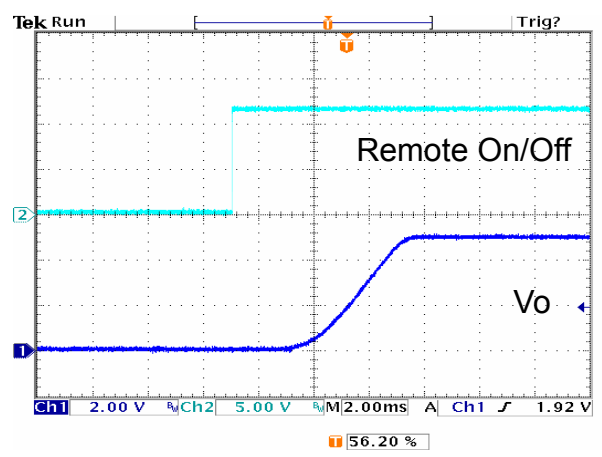
Figure 12: Turn on delay by Remote On/Off, 5.0V/20A out
