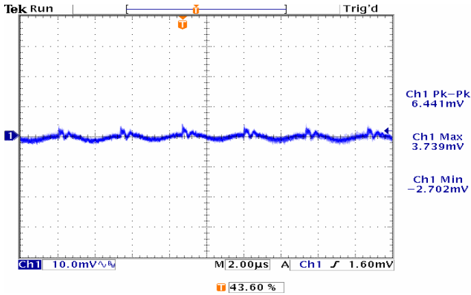
Figure 7: Output ripple & noise at 12Vin, 0.7525V/20A out
