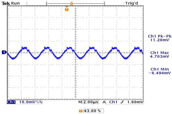
Figure 9: Output ripple & noise at 12Vin, 2.5V/20A out
