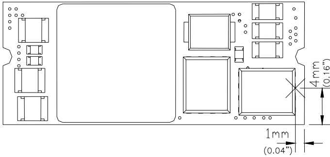
Figure 39: Temperature measurement location
