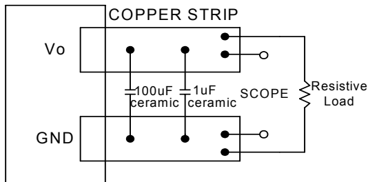
Figure 25: Input reflected-ripple test setup
