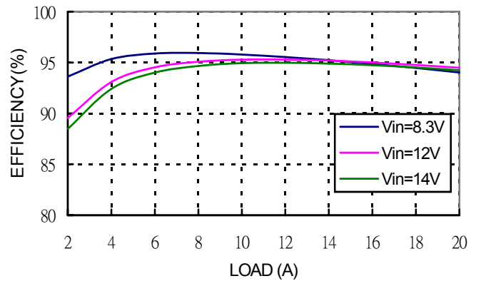
Figure 6: Converter efficiency vs. output current (5.0V output voltage)
