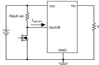
Figure 30: Negative remote On/Off implementation
