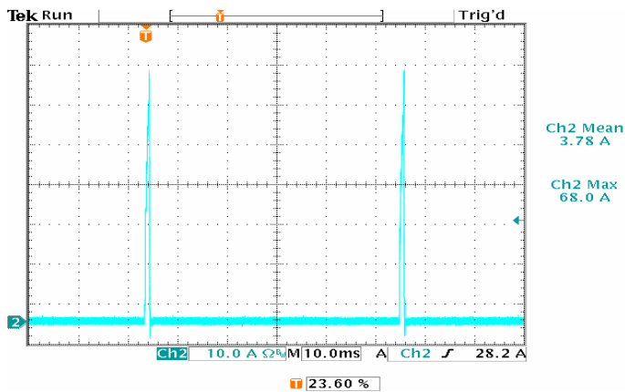
Figure 23: Output short circuit current 12V_{in} , 0.75V_{out} ( 10A/div )
