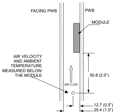
Note: Wind Tunnel Test Setup Figure Dimensions are in millimeters and (Inches) Figure 44: Wind tunnel test setup
