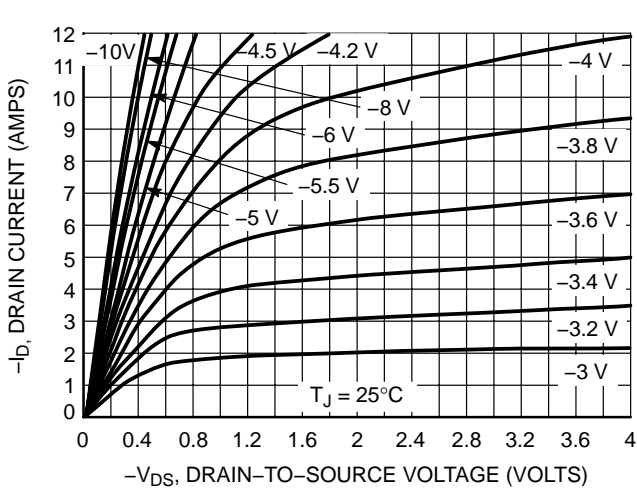
Figure 4. On-Region Characteristics
