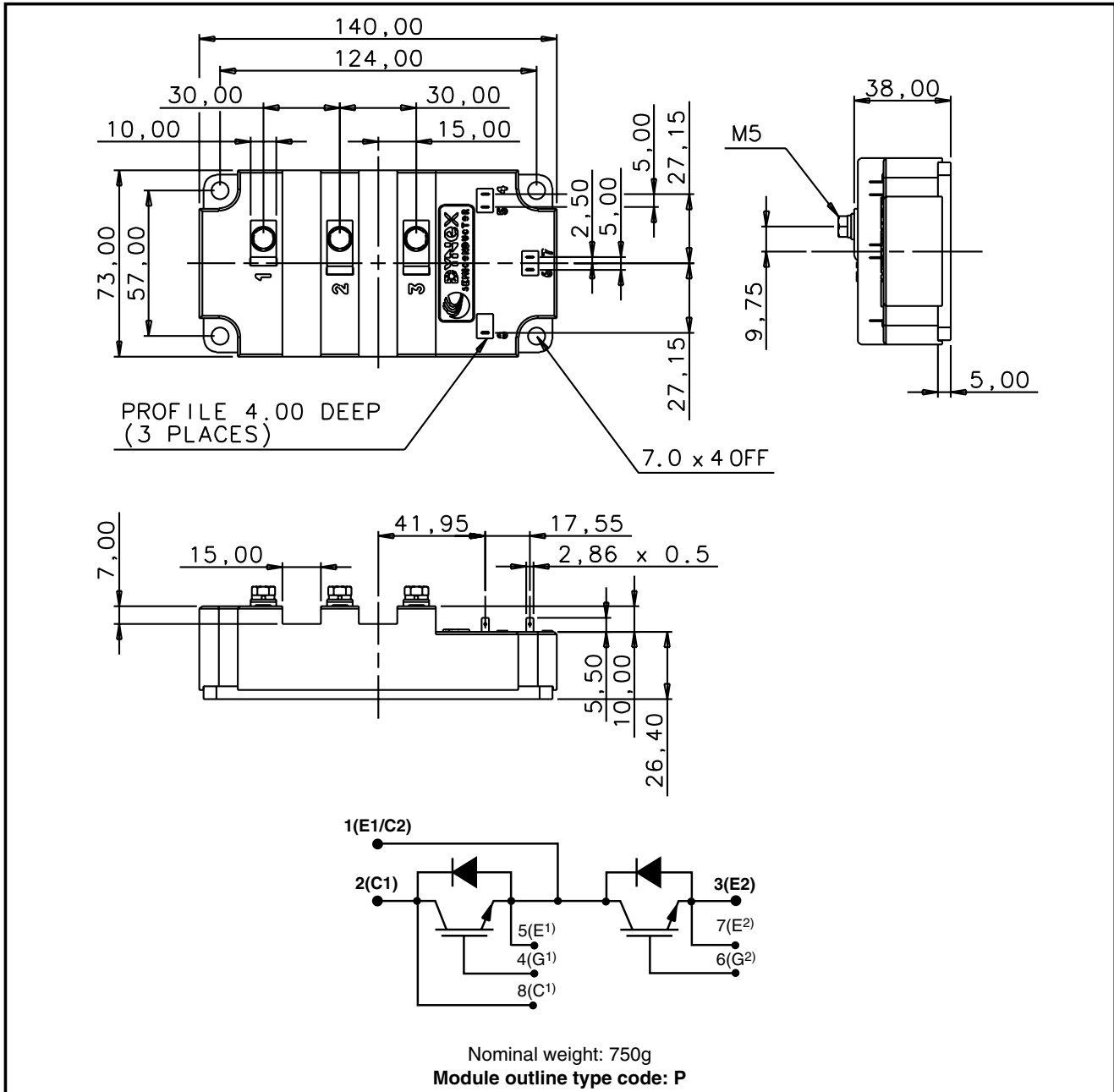
Fig. 11 Package details
