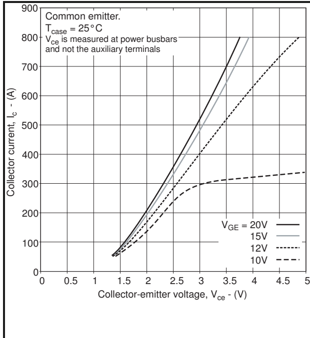
Fig.3 Typical output characteristics @ 25°C
