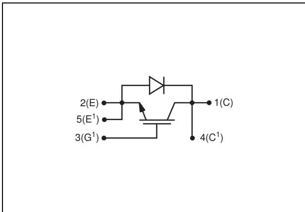
Fig. 1 Single switch circuit diagram
