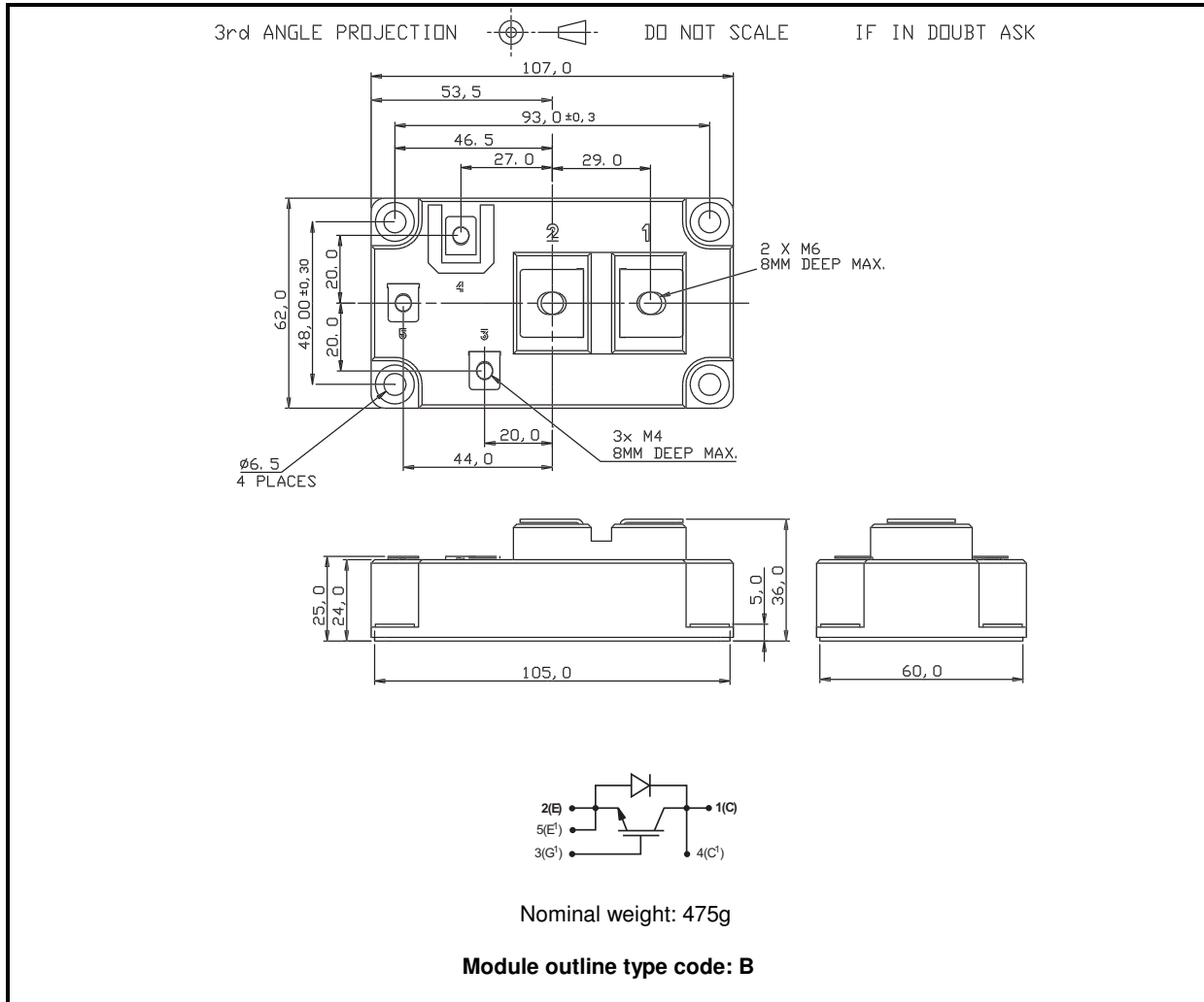
Fig.11 Package details
