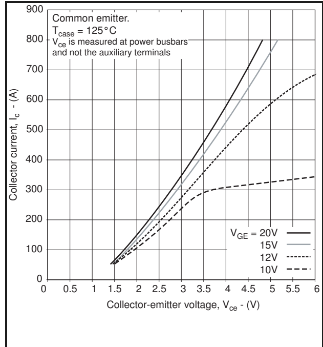
Fig.4 Typical output characteristics @ 125°C
