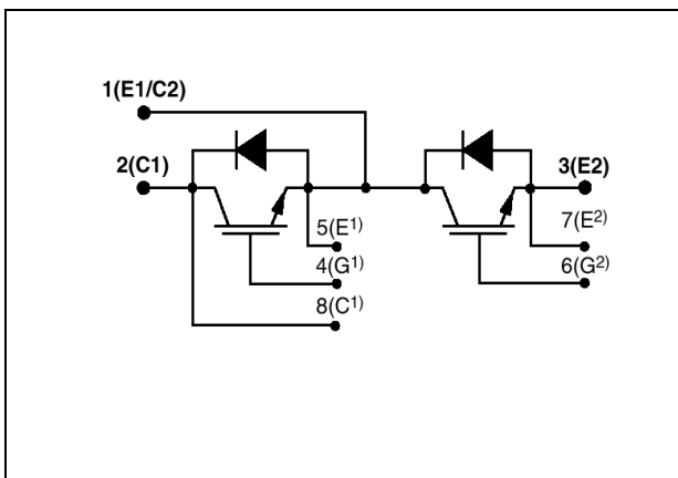
Fig. 1 Half Bridge circuit diagram
