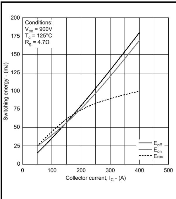
Fig.5 Typical switching energy vs collector current
