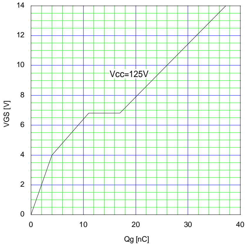
Typical Gate Charge Characteristics V_{GS} = f(Q_g) : I_D = 18.0 A, T_{ch} = 25 \text{ } ^\circ C
