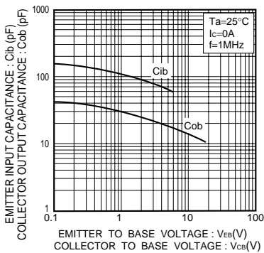
Fig.7 Collector output capacitance vs. collector-base voltage vs. emitter input capacitance vs. emitter-base voltage
