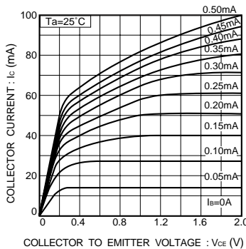
Fig.11 Grounded emitter output characteristics ( I )
