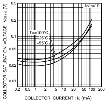
Fig.16 Collector-emitter saturation voltage vs. collector current ( II )
