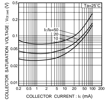
Fig.15 Collector-emitter saturation voltage vs. collector current ( I )
