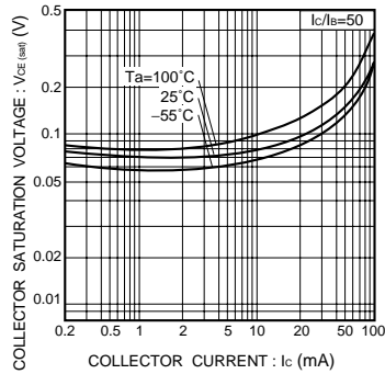
Fig.17 Collector-emitter saturation voltage vs. collector current ( III )
