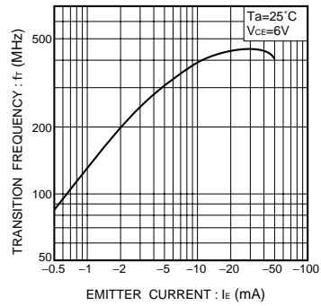
Fig.18 Gain bandwidth product vs. emitter current
