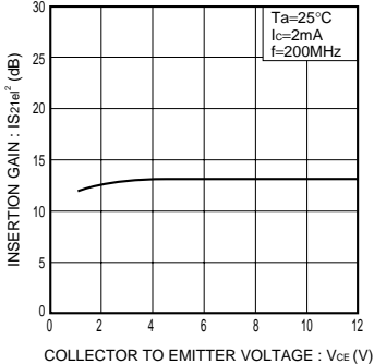
Fig.8 Insertion gain vs. collector voltage
