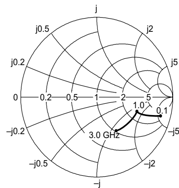
Figure 9. Output Reflection Coefficient
