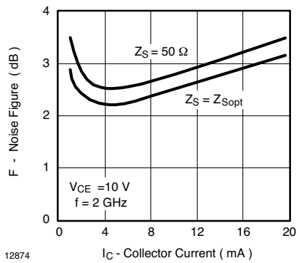
Figure 5. Noise Figure vs. Collector Current
