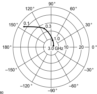
Figure 8. Forward Transmission Coefficient
