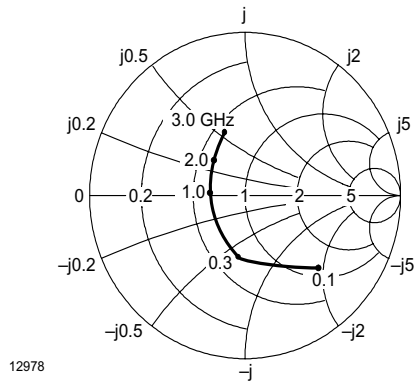
Figure 6. Input Reflection Coefficient
