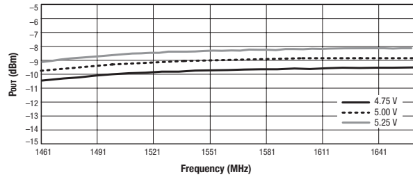
Figure 11. Output Power vs Frequency and Supply Voltage
