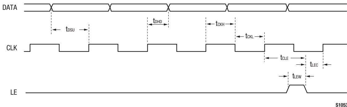
Figure 3. SKY73103-11 Serial Data Input Timing Diagram (MSB First)
