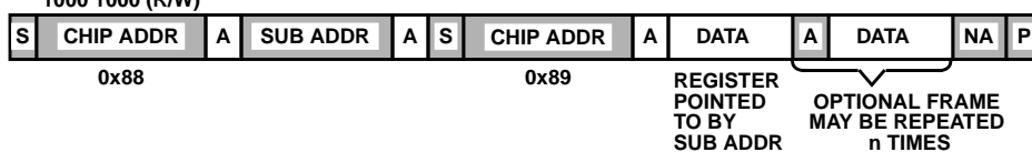
FIGURE 21. REGISTER WRITE/READ FLOW
