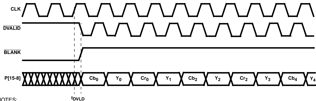
FIGURE 10. OUTPUT TIMING FOR 8-BIT YCbCr MODE (DVLD_LTC = 0)
