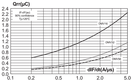
Fig. 6-1: Reverse recovery charges versus dI_F/dt (damper diode).
