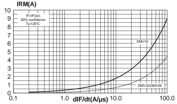
Fig. 7-2: Reverse recovery current versus dI_F/dt (modulation diode).
