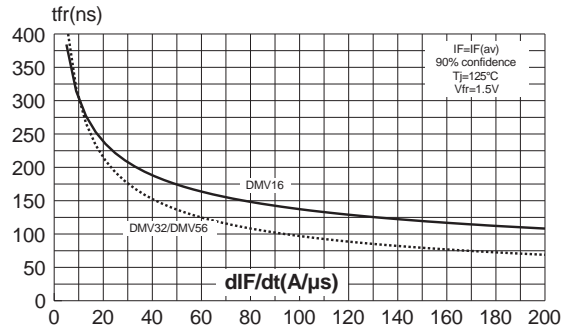
Fig. 9-2: Forward recovery time versus dI_F/dt (modulation diode).
