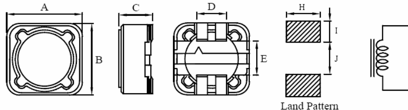
Land Pattern
