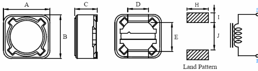
Land Pattern
