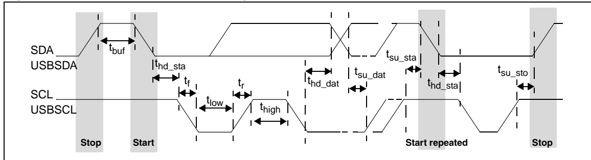
Figure 8. Control interface: I2C timing
