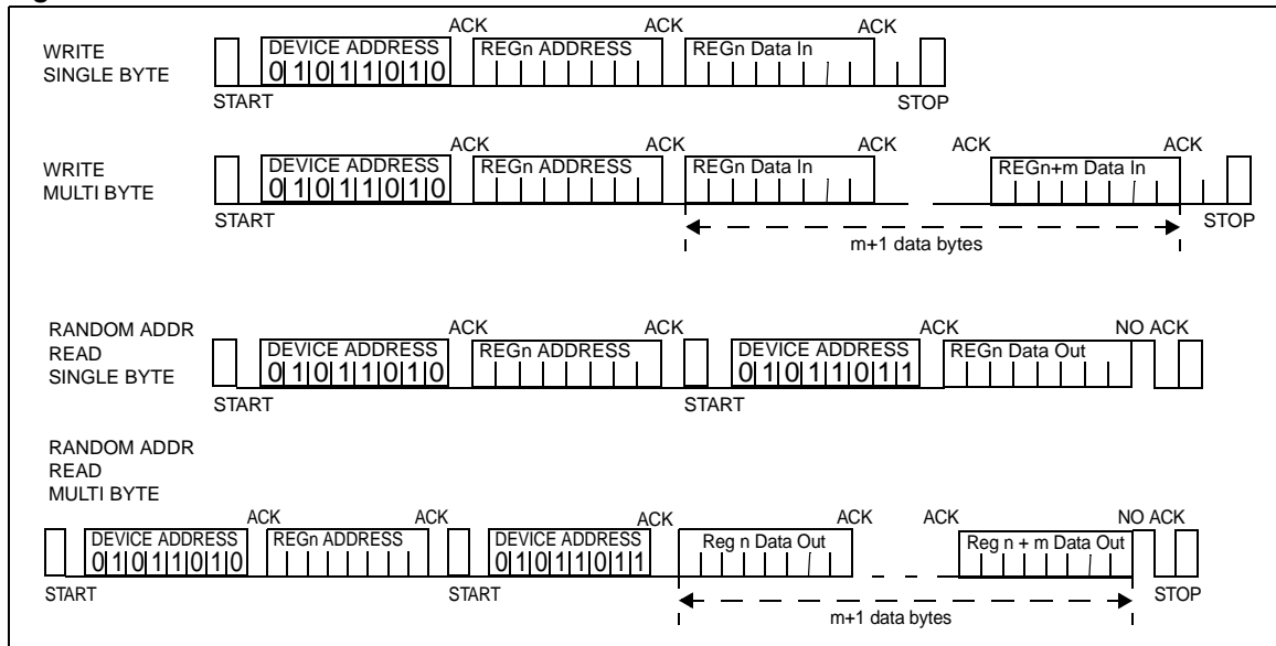
Figure 7. Control interface: I2C format
