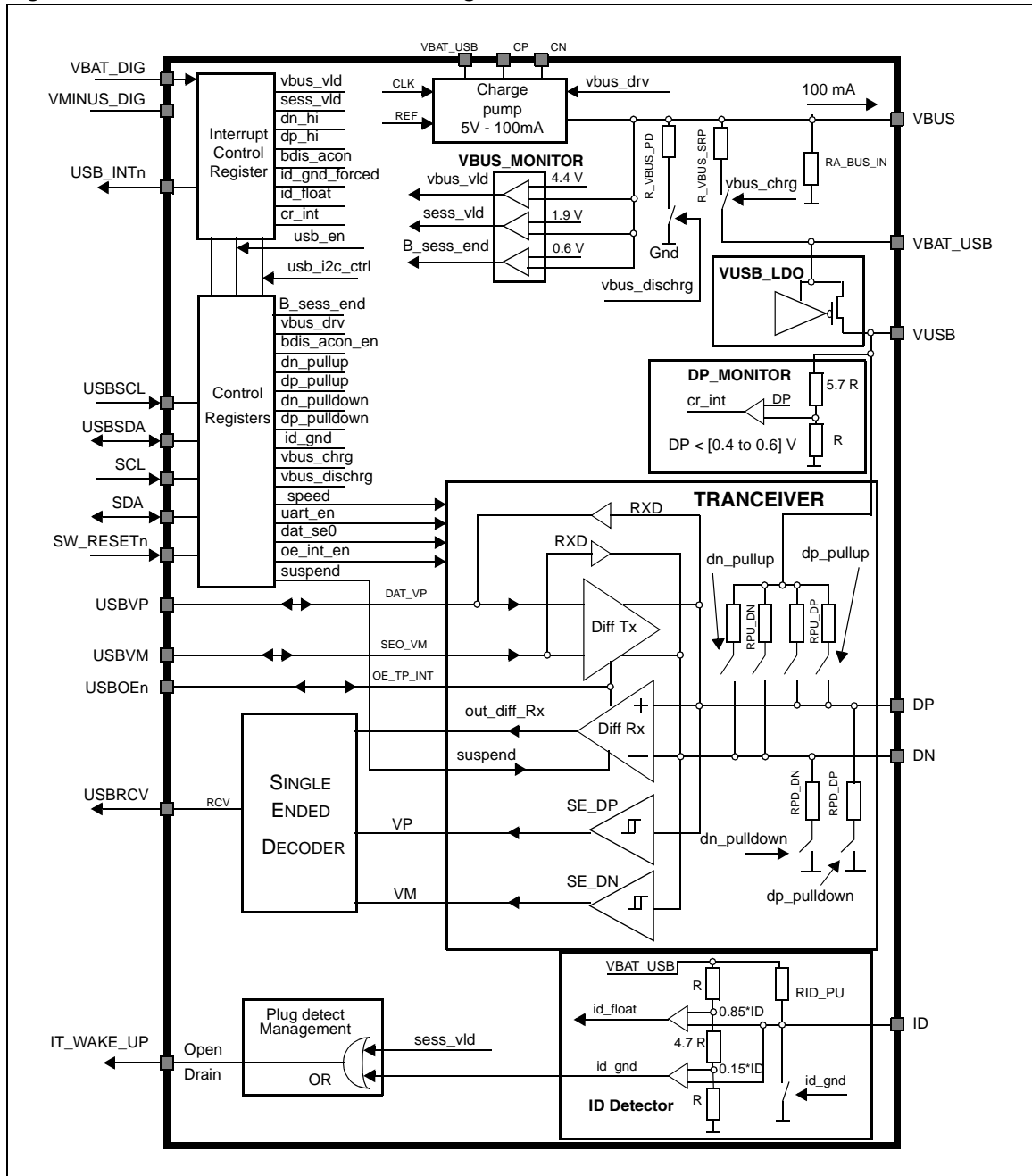
Figure 13. USB OTG transceiver block diagram
