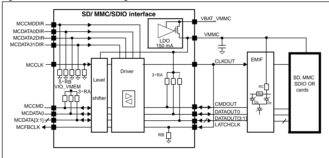
Figure 14. SD/MMC/SDIO block diagram
