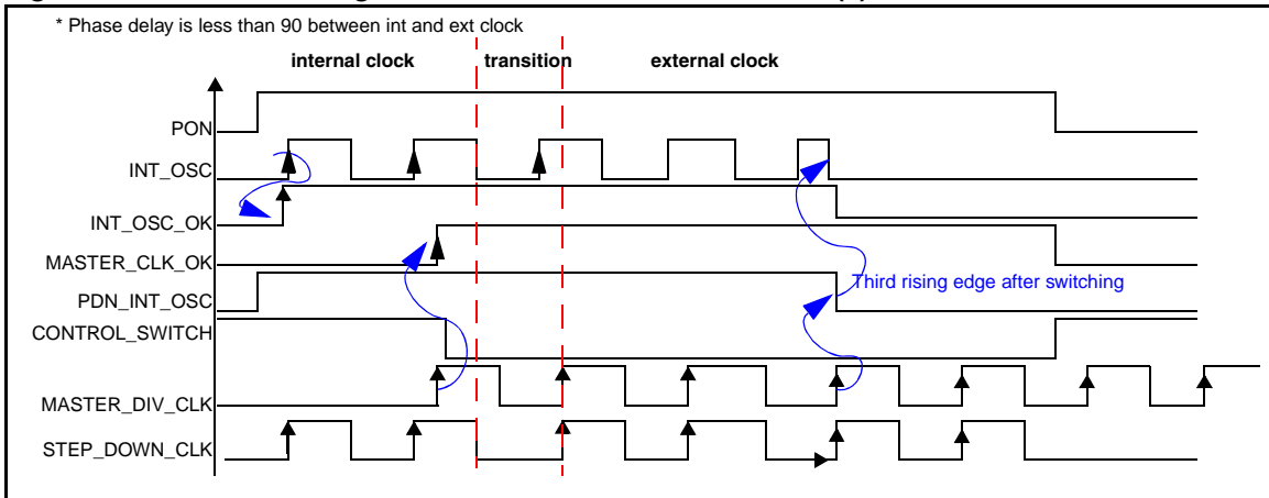
Figure 9. Clock switching between master and internal clock (1)
