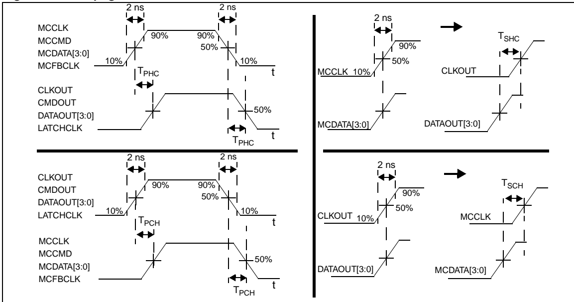
Figure 15. Propagation and clock/data skew times
