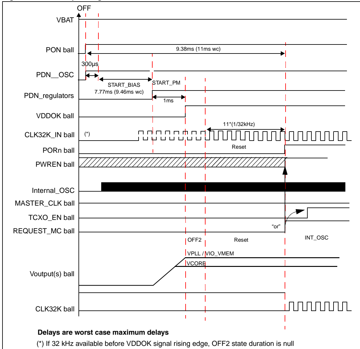
Figure 3. Start-up timing
