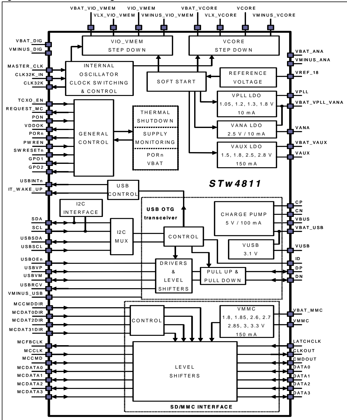
Figure 2. STw4811 block diagram
