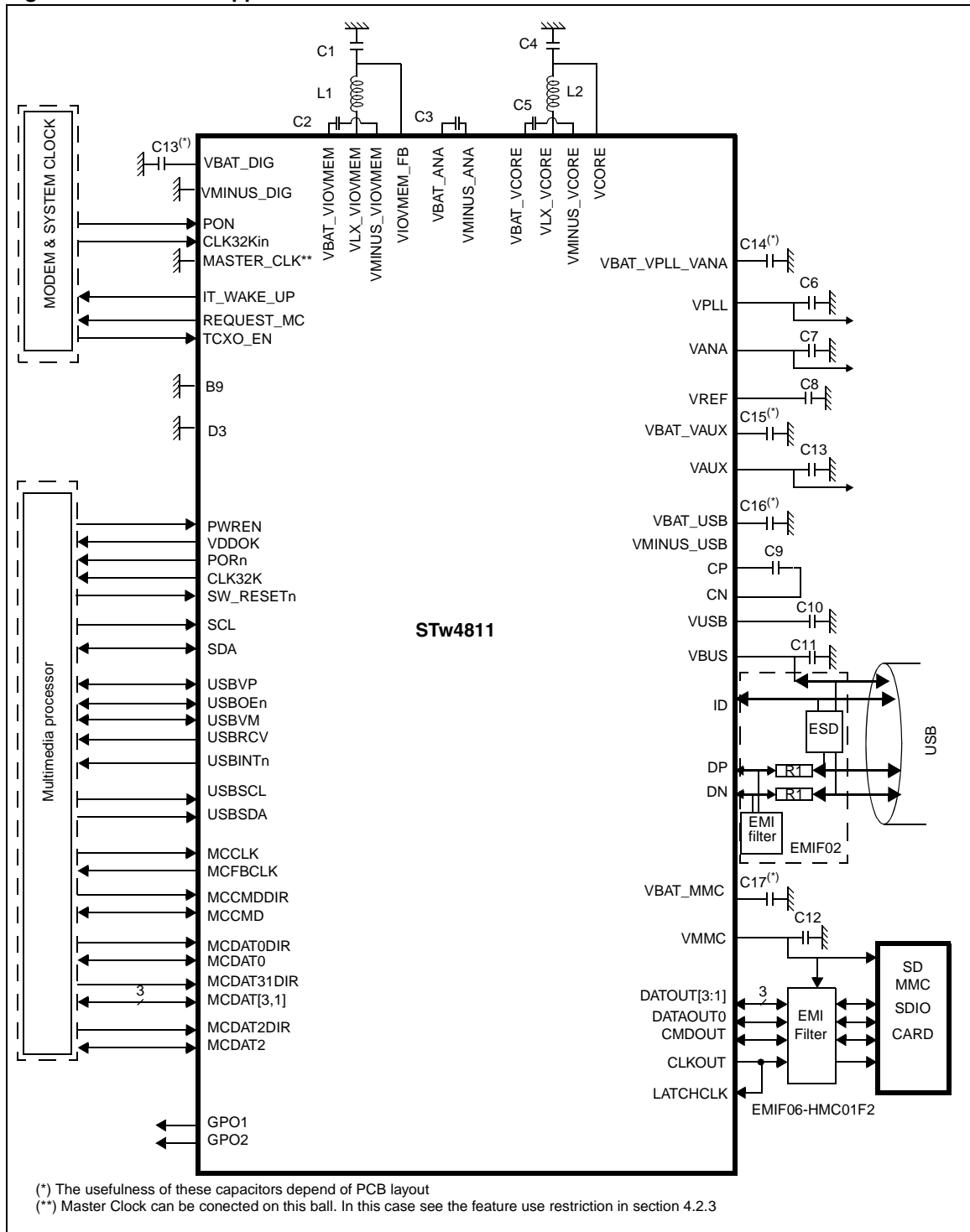
Figure 16. STw4811 application schematics
