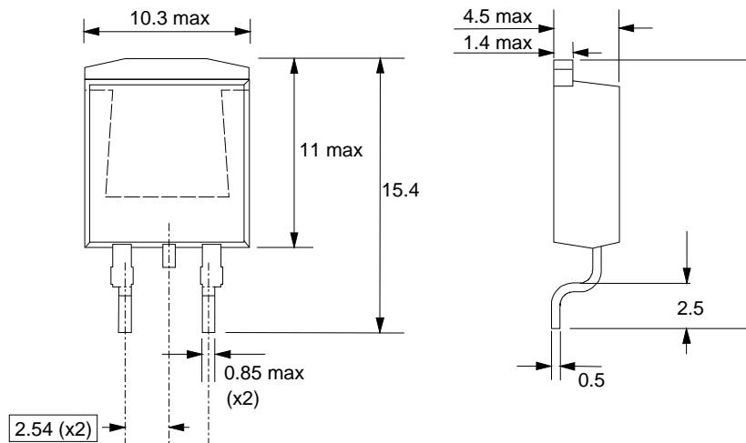
Fig.19. SOT404 : centre pin connected to mounting base.
