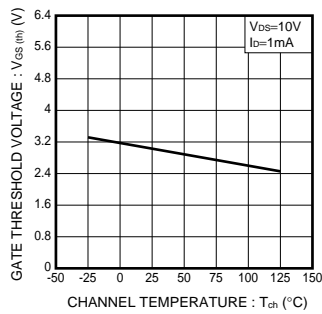
Fig.4 Gate Threshold Voltage vs. Channel Temperature
