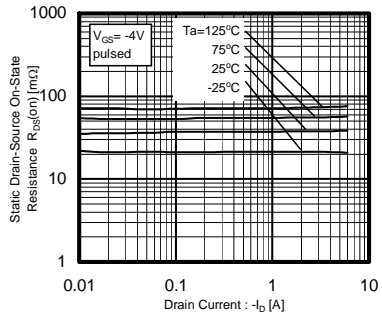
Fig.4 Static Drain-Source On-State Resistance vs. Drain Current (3)
