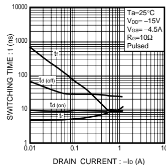
Fig.8 Switching Characteristics
