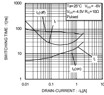
Fig.12 Switching Characteristics
