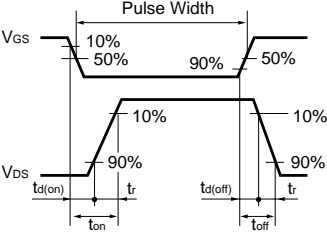
Fig.11 Switching Waveforms
