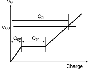
Fig.13 Gate Charge Waveforms
