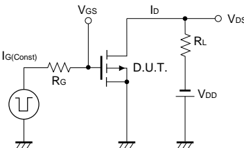
Fig.12 Gate Charge Measurement Circuit
