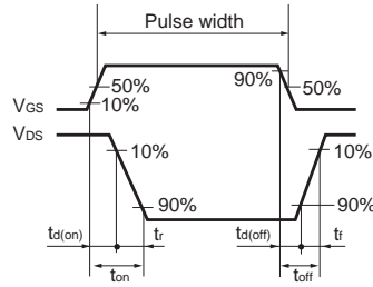
Fig.1-2 Switching waveforms
