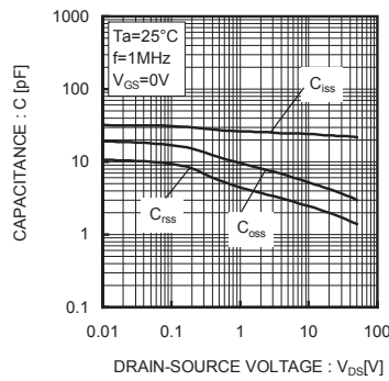
Fig.14 Typical Capacitance vs. Drain-Source Voltage
