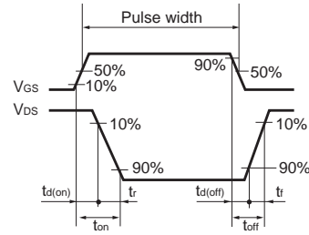
Fig.1-2 Switching waveforms
