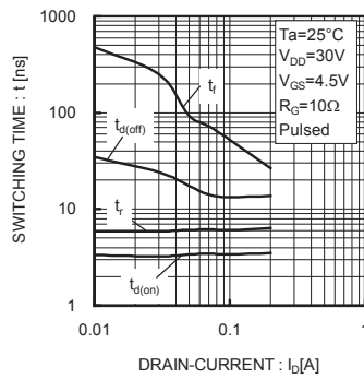
Fig.13 Switching Characteristics
