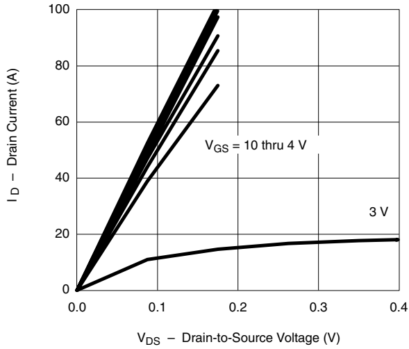
V_{GS} = 10 thru 4 V 3 V Output Characteristics
