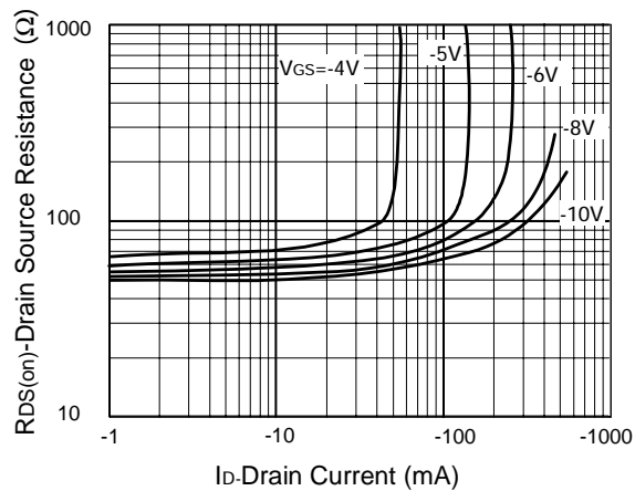
On-resistance v Gate-Source Voltage
