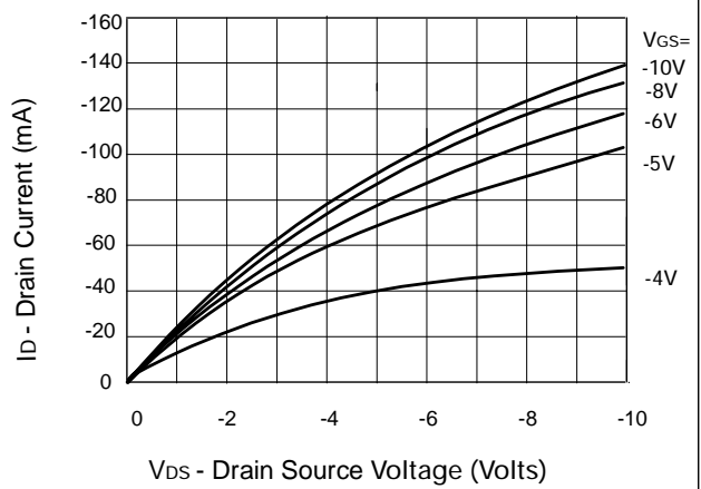
Saturation Characteristics
