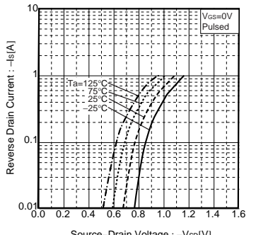
Fig.7 Reverse Drain Current vs. Source-Drain Current
