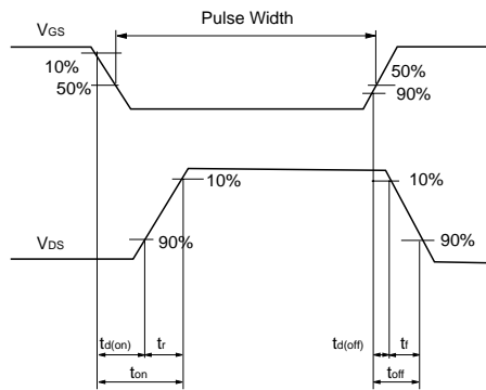
Fig.14 Switching Waveforms
