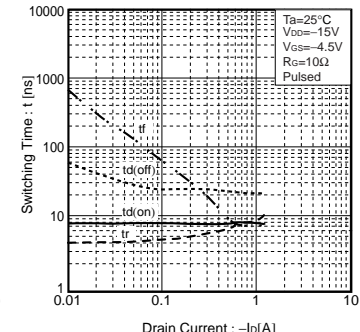
Fig.9 Switching Characteristics
