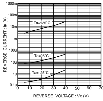
Fig.9 Reverse characteristics
