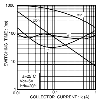
Fig.6 Switching time
