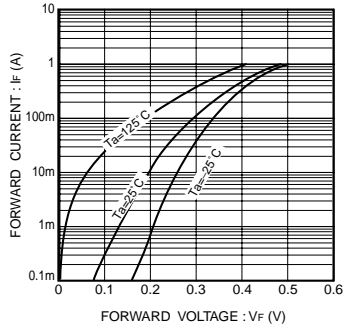
Fig.8 Forward characteristics
