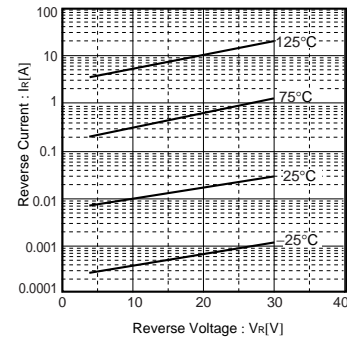
Fig.12 Reverse Temperature Characteristics
