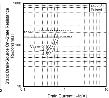
Fig.6 Static Drain-Source On-State Resistance vs. Drain Current
