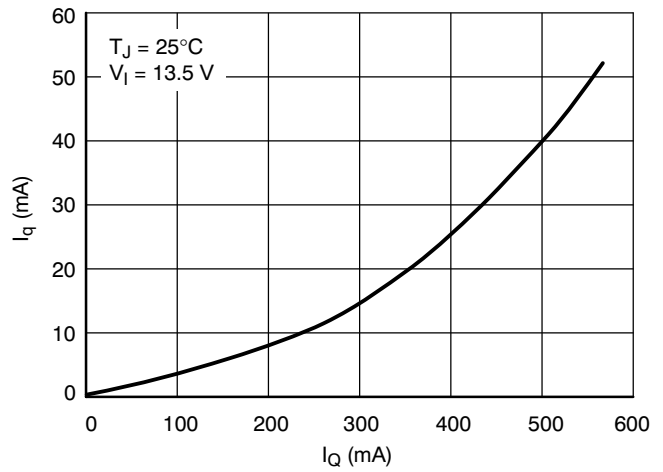
Figure 16. Current Consumption vs. Output Current (High Load)
