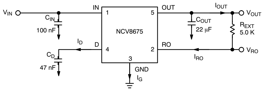
Figure 34. Application Circuits
