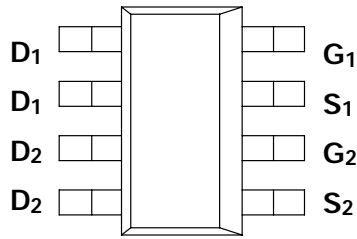
PARTMARKING DETAIL - M4306N
